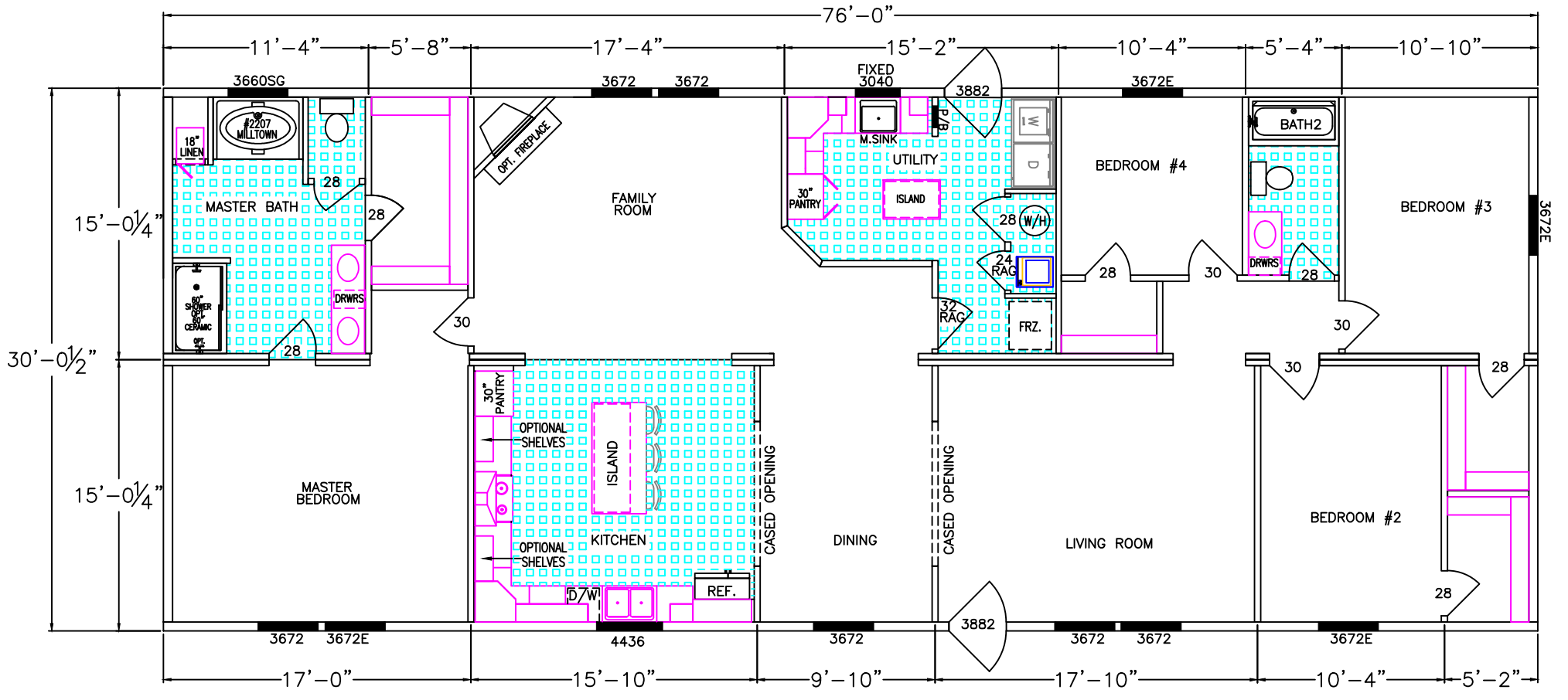
"KYLEIGH" ESSENTIAL***622-80-4-32 (APPROXIMATELY 2280 SF)
