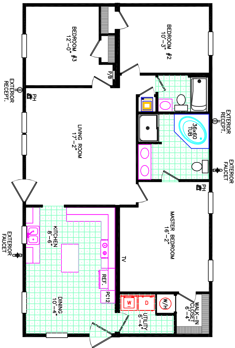
2002-52-3-30 30 x 52 3 BEDROOM 2 BATH (APPROXIMATELY 1814 SF )
